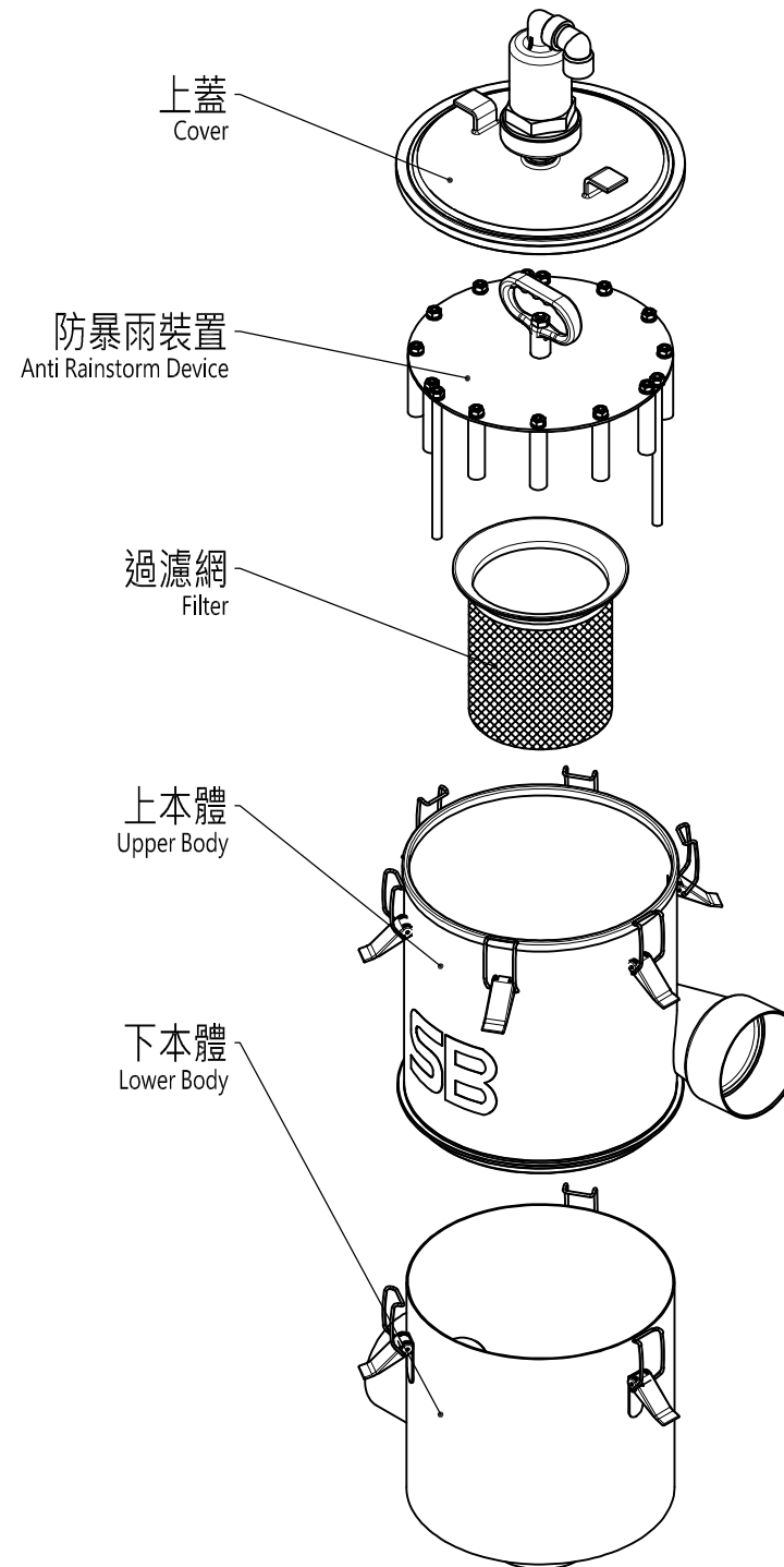
雨水回收過濾器分解圖 Rainwater Filter Exploded Diagram
